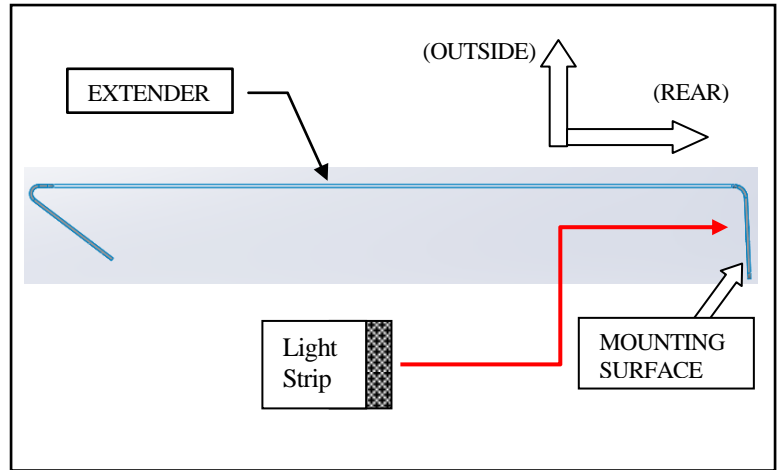
Figure 2 Installation Direction
